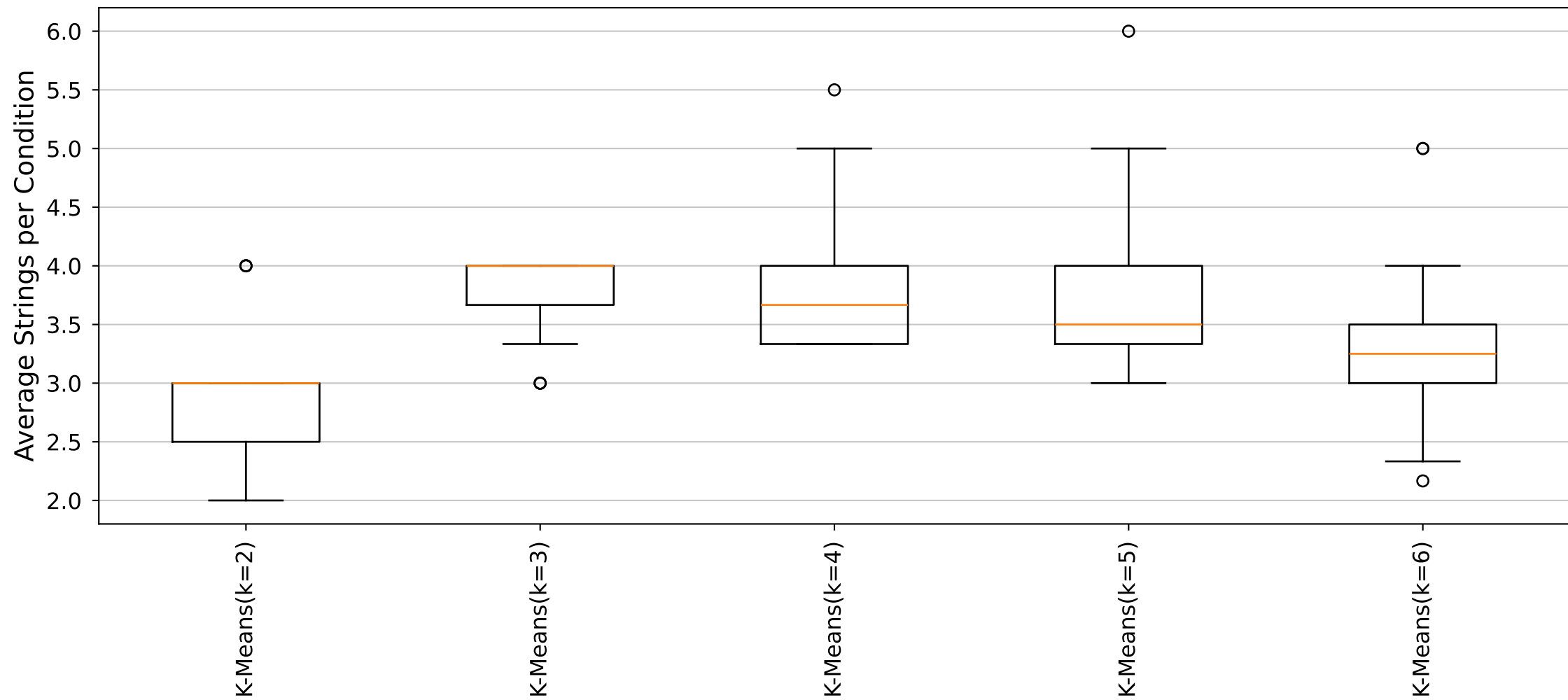
YARA Rules Average Strings per Condition Distribution (Cluster23_Size6 dataset)
